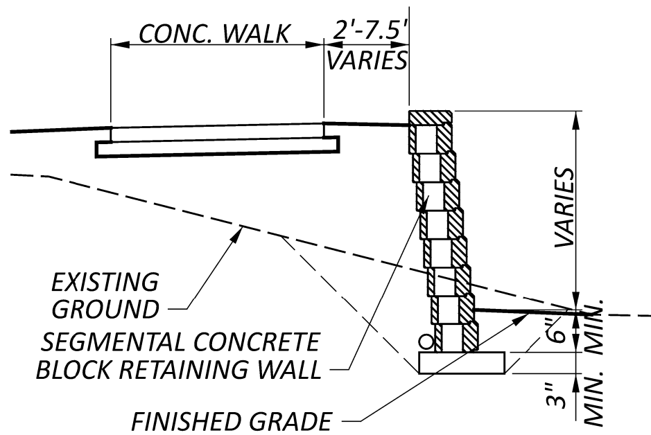
TYPICAL WALL SECTION NOT TO SCALE
