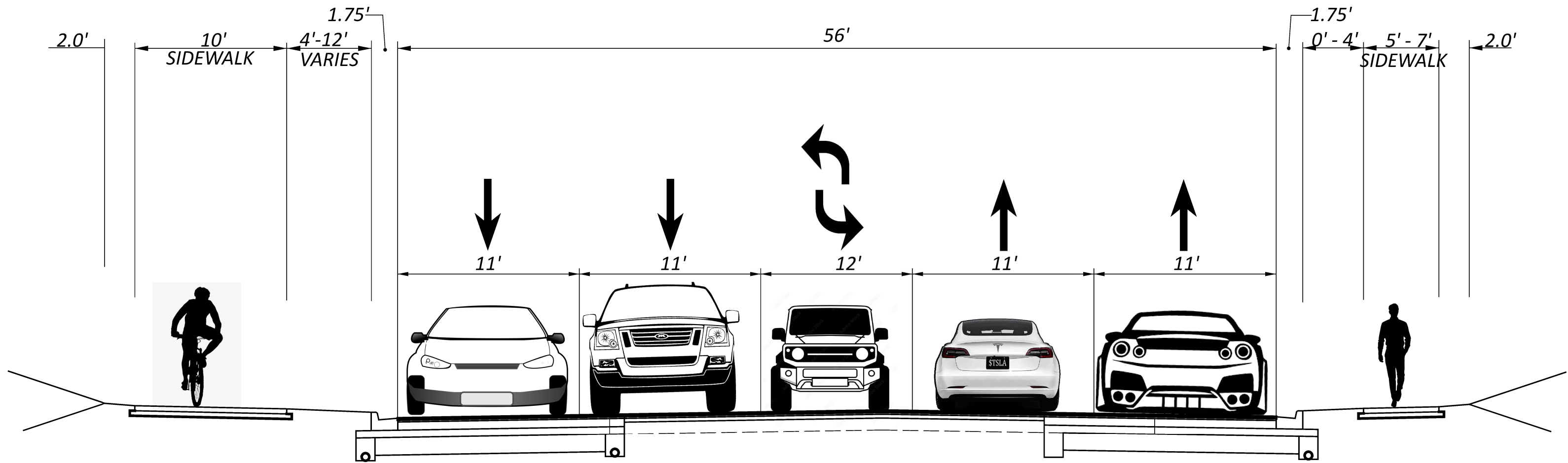
TYPICAL SECTION - CR 142 ( MEADOW BRIDGE DR. - HIGHVIEW DR.) NOT TO SCALE
