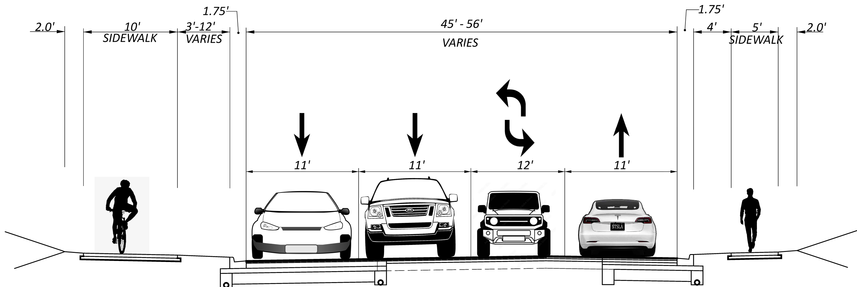
TYPICAL SECTION - CR 142 ( HIGHVIEW DR. - DARLINGTON DR.) NOT TO SCALE
